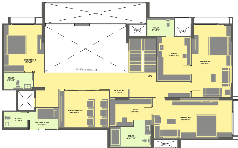
BLOCK B & C Duplex Upper Level Plan
