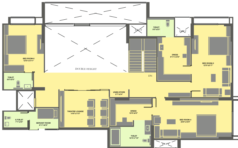
BLOCK B & C Triplex Middle Level Plan
